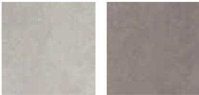
argilla
